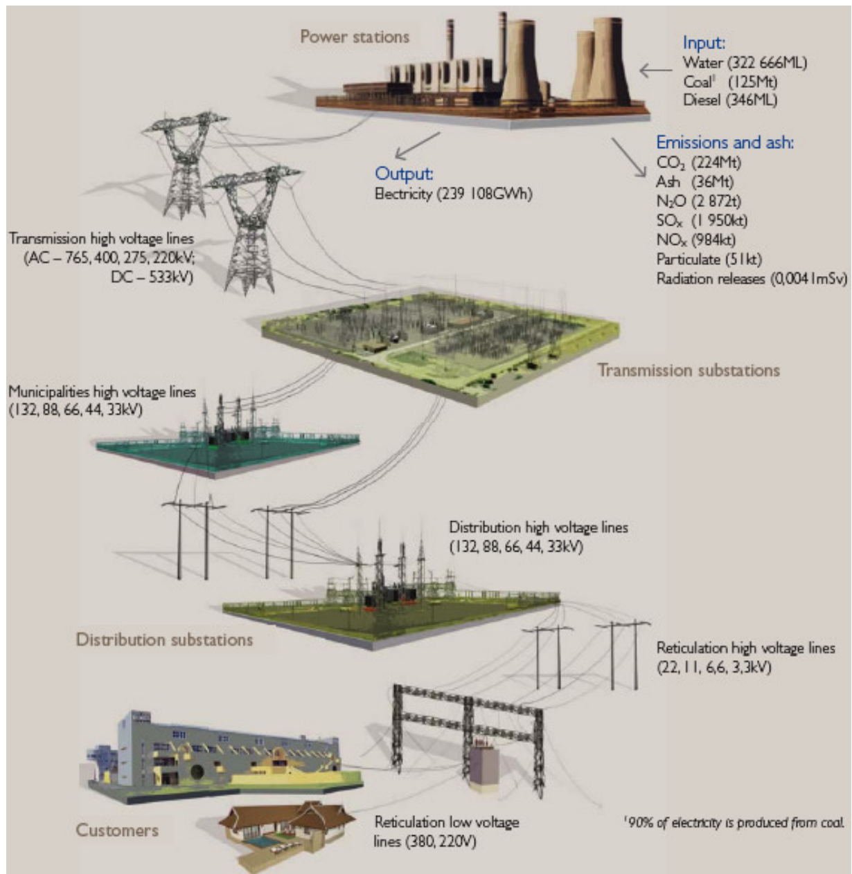
Figure 3.1: Simplified electrical transmission and distribution system (source: www.eskom.co.za)
