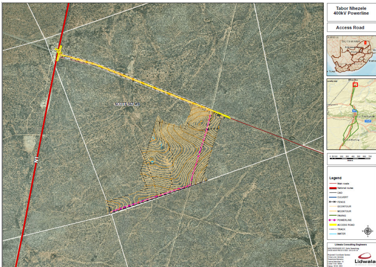
Figure 3.8: Access road proposed between the N1 and the Nzhelele substation
