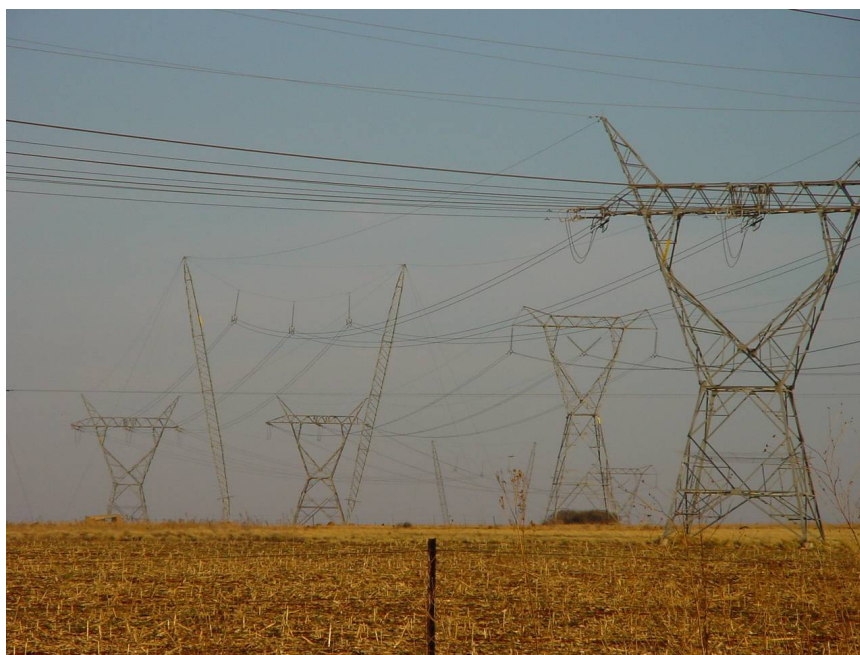
Figure 3.2: Photograph of Self-supporting Strain tower (in foreground) and Cross Rope Suspension tower (in centre) designs.
